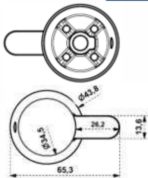
Centre Handle FC | FSN Centre 60 58 gms
