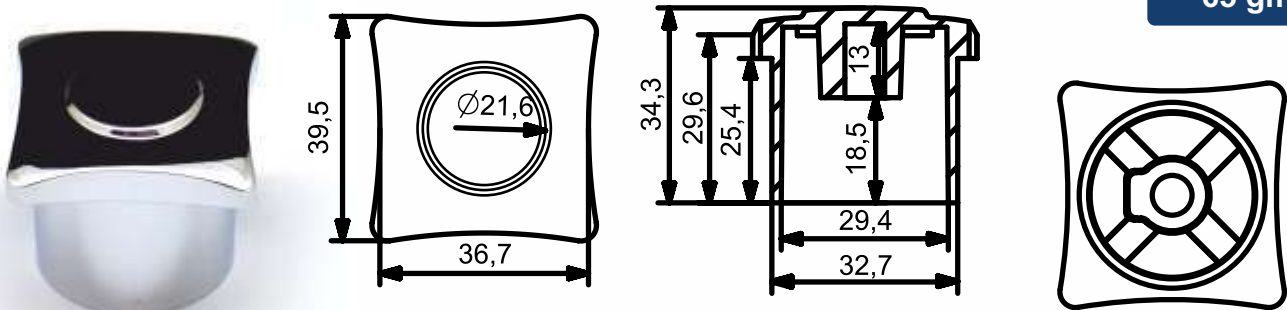
Square F 65 | SQF 65 65 gms
