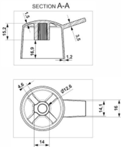
Centre Handle Ocean 60 | CHO 60 60 gms
