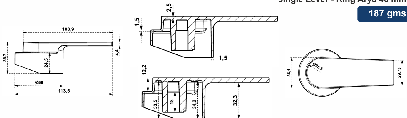
Single Lever - King Arya 45 mm
