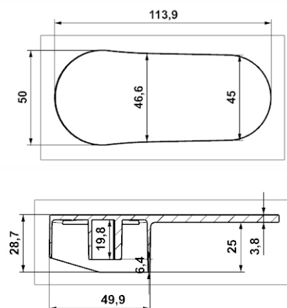
Single Lever - Opel 40 mm
