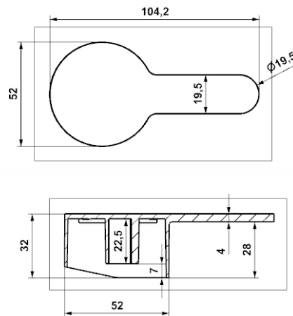
Single Lever - Fusion 40 mm
