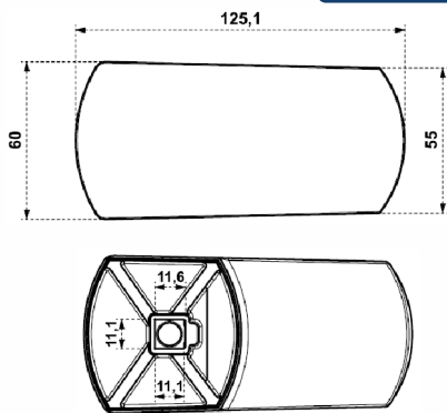
Single Lever - Kubix Prime 46 mm
