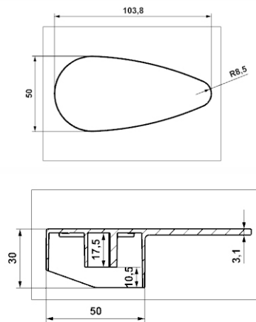
Single Lever - Vignet 40 mm
