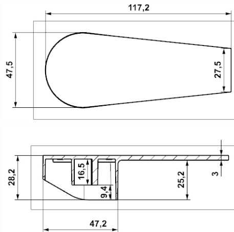
Single Lever - Arya 40 mm
