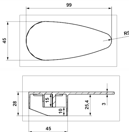
Single Lever - Vignet 35 mm
