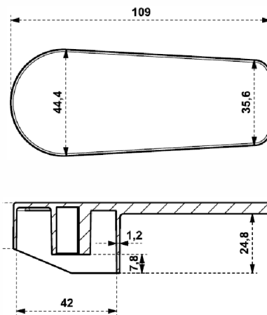
Single Lever - Punch 35 mm
