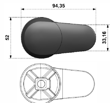
Single Lever - Ronja 40mm
