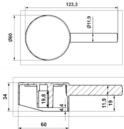
Single Lever - Turbo 45 mm
