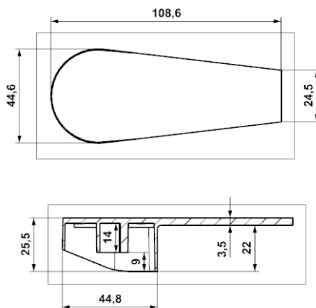
Single Lever - Arya 35 mm
