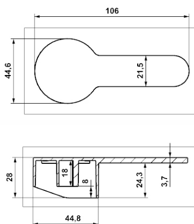
Single Lever - Fusion 35 mm
