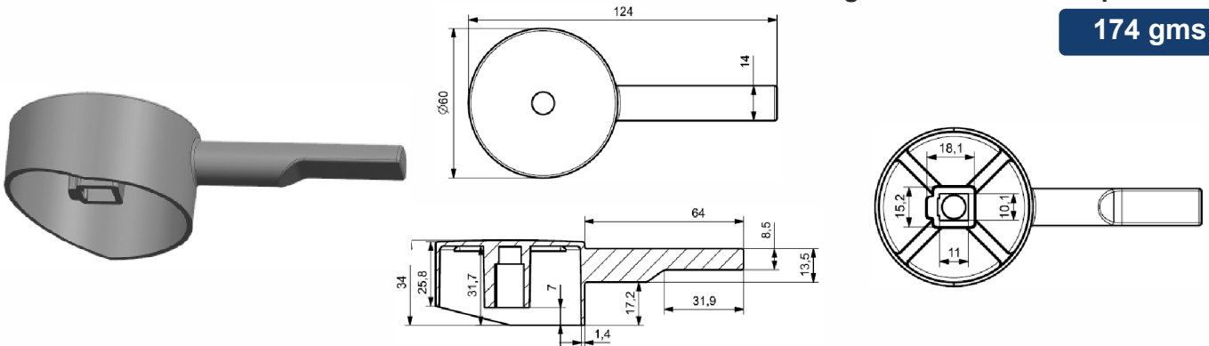
Single Lever - Turbo Step 45 mm
