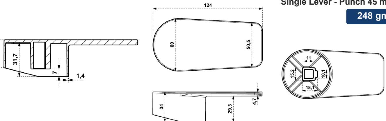
Single Lever - Punch 45 mm
