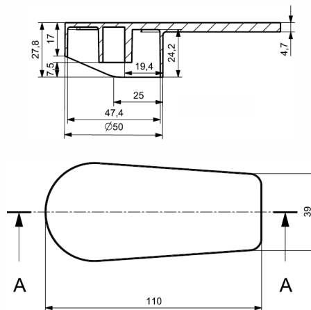
Single Lever - Punch 40 mm
