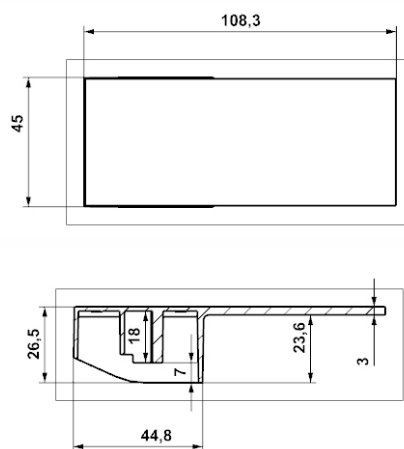
Single Lever - Cubix 35 mm
