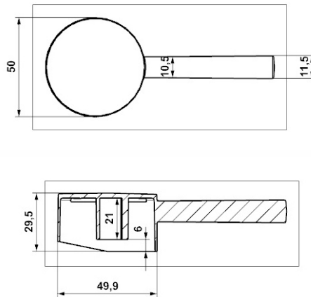
Single Lever - Turbo 40 mm
